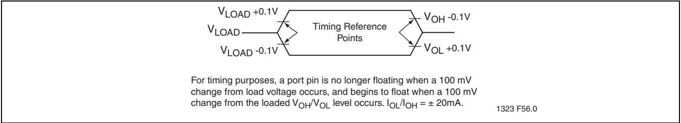
FIGURE 12-6: Float Waveform
