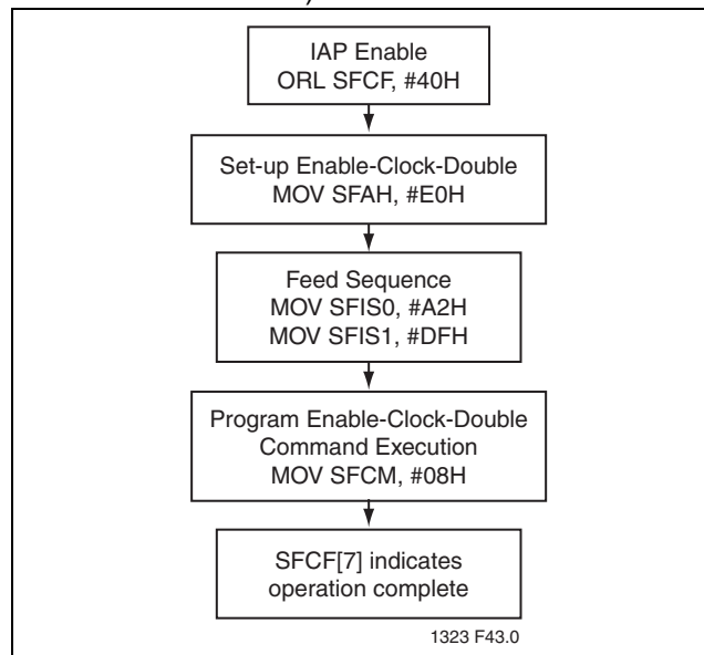
FIGURE 4-7: Enable-Clock-Double
