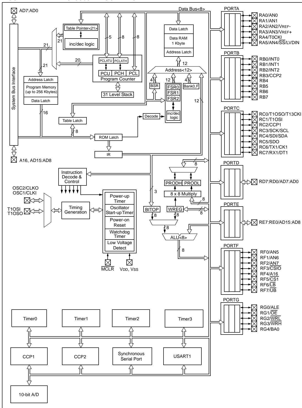
FIGURE 1-1: PIC18C601 BLOCK DIAGRAM
