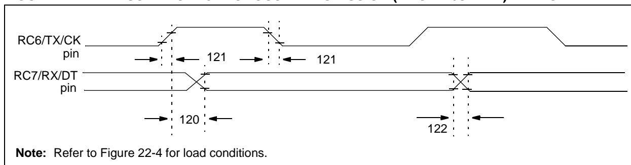
FIGURE 22-21: USART SYNCHRONOUS TRANSMISSION (MASTER/SLAVE) TIMING
