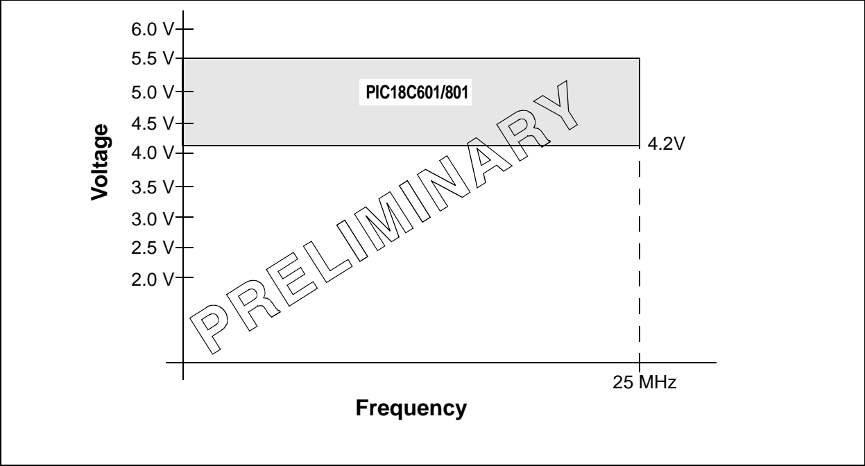
FIGURE 22-2: PIC18C601/801 VOLTAGE-FREQUENCY GRAPH (EXTENDED)
