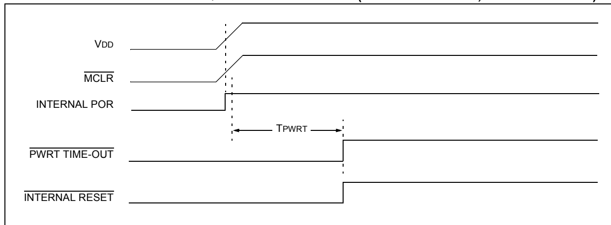
FIGURE 5-3: TIME-OUT SEQUENCE ON POWER-UP ( \overline{\text{MCLR}} TIED TO \text{V}_{\text{DD}} , \text{V}_{\text{DD}} \text{ RISE} < \text{TPWRT} )
