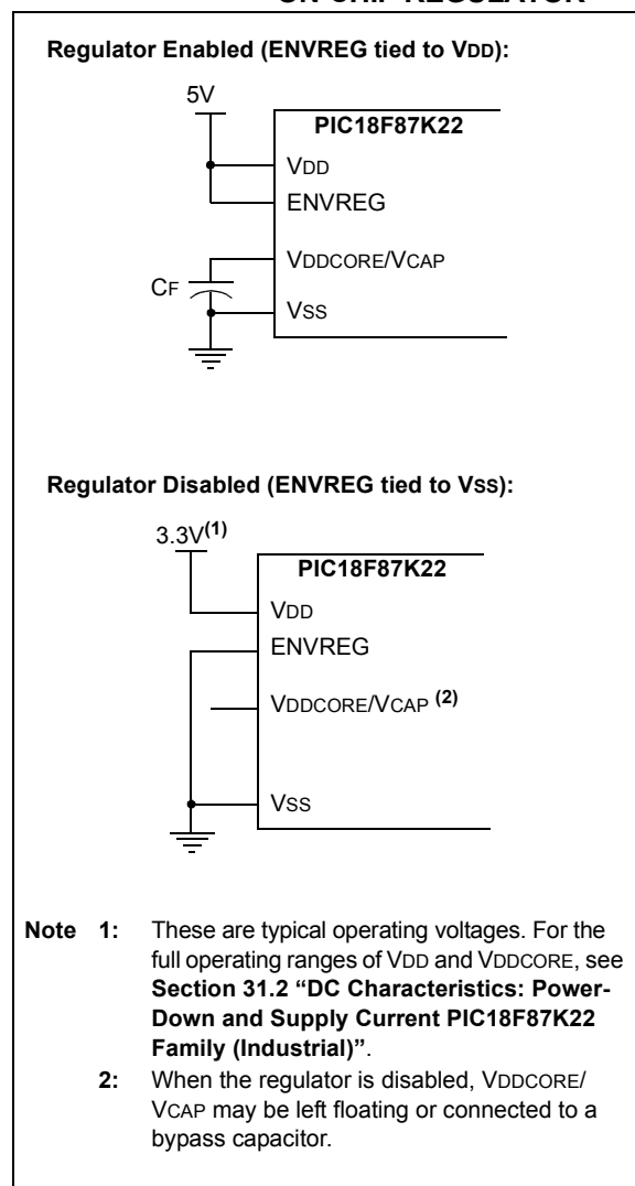
FIGURE 28-2: CONNECTIONS FOR THE ON-CHIP REGULATOR
