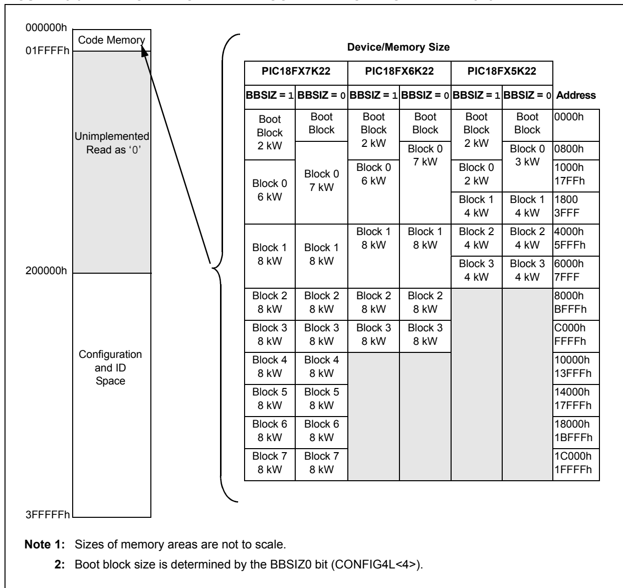
FIGURE 28-6: CODE-PROTECTED PROGRAM MEMORY FOR THE PIC18F87K22 FAMILY
