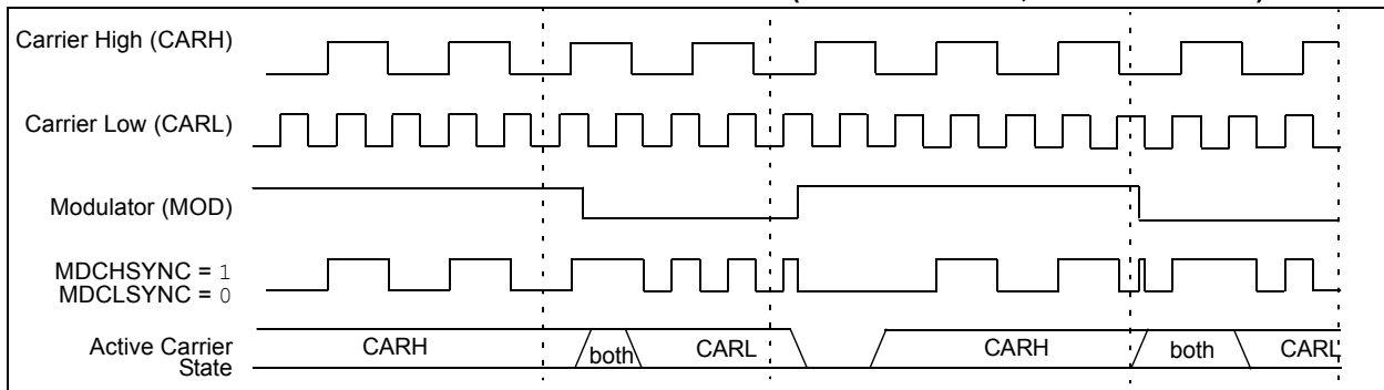
FIGURE 22-3: CARRIER HIGH SYNCHRONIZATION (MDCHSYNC = 1, MDCLSYNC = 0)
