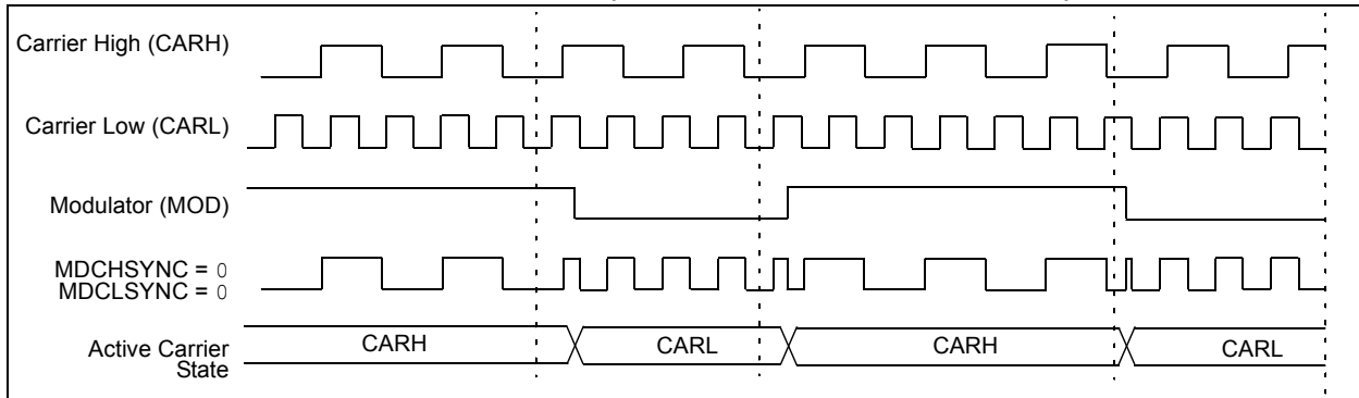
EXAMPLE 22-1: NO SYNCHRONIZATION (MDCHSYNC = 0, MDCLSYNC = 0)
