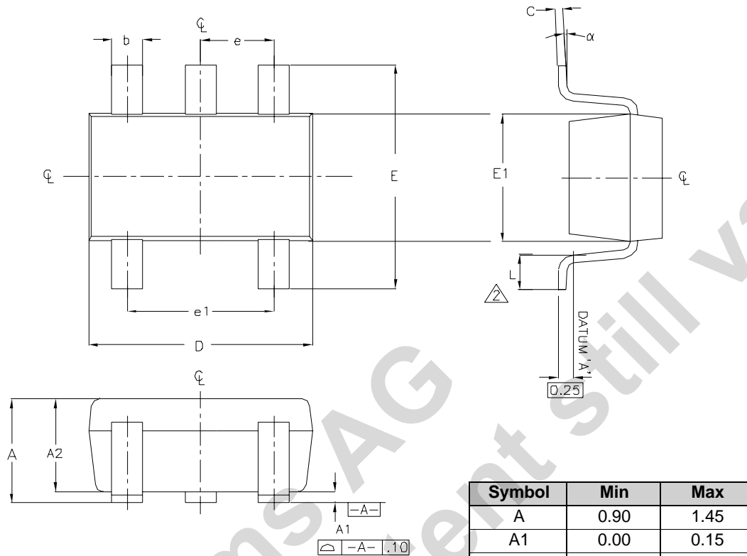
Figure 15. 5-pin SOT23 Package
