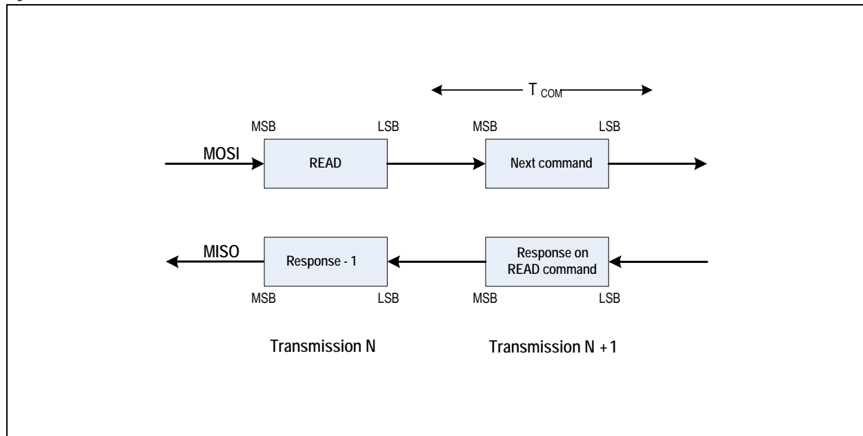
Figure 5. READ Command
