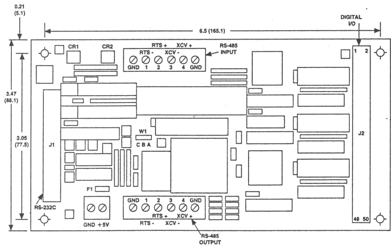
Figure 5. Outline Dimensions
