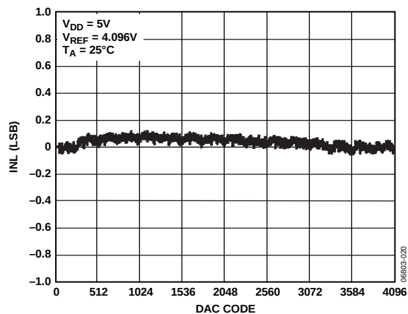
Figure 9. AD5044 INL
