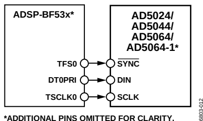
Figure 52. AD5024/AD5044/AD5064/AD5064-1 to Blackfin ADSP-BF53x Interface
