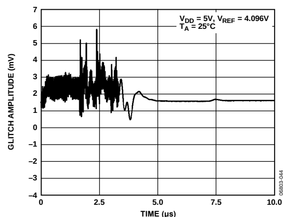
Figure 33. DAC-to-DAC Crosstalk
