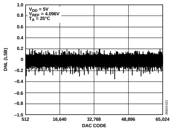
Figure 11. AD5064/AD5064-1 DNL
