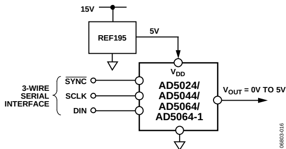
Figure 56. REF195 as Power Supply to the AD5024/AD5044/AD5064/AD5064-1
