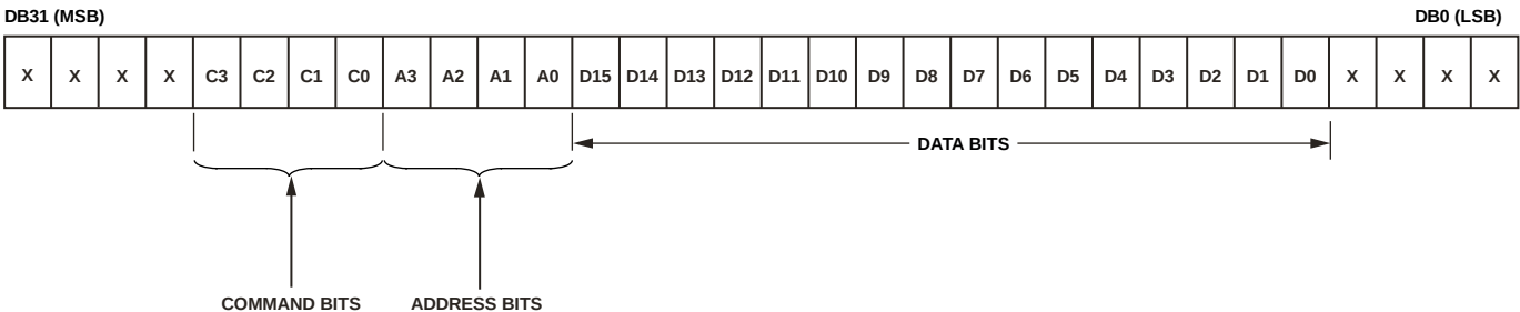
Figure 49. AD5064/AD5064-1 Shift Register Content
