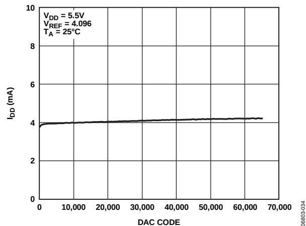
Figure 23. Supply Current vs. Code
