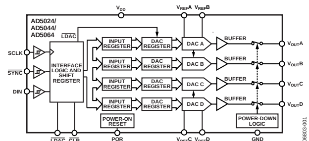
Figure 2. AD5024/AD5044/AD5064 with Individual Reference Pins
