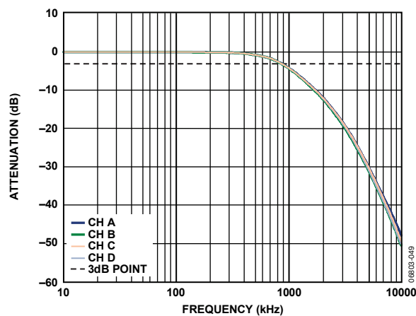
Figure 38. Multiplying Bandwidth
