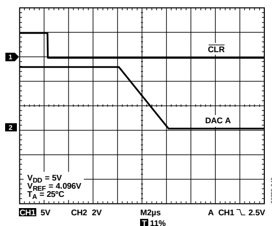
Figure 37. Hardware \overline{CLR}
