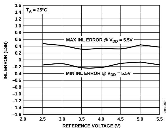
Figure 15. INL vs. Reference Input Voltage
