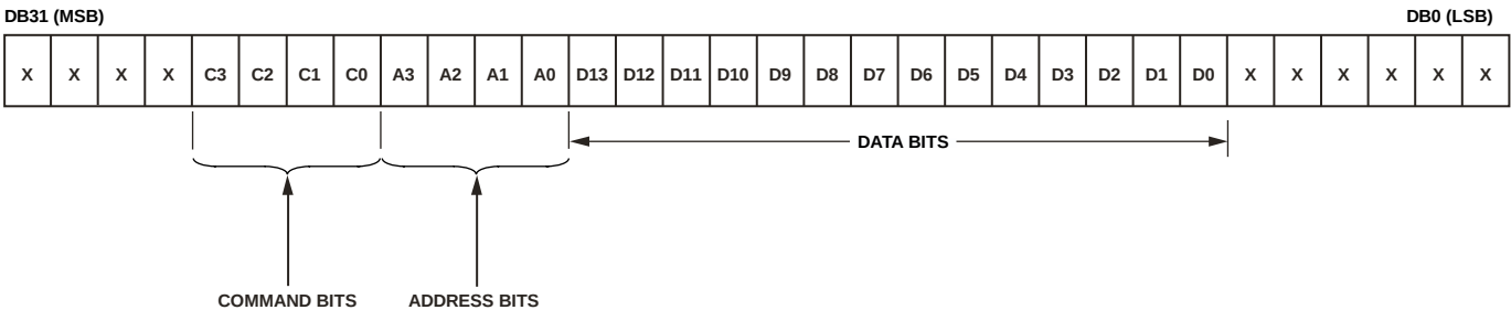
Figure 48. AD5044 Shift Register Content
