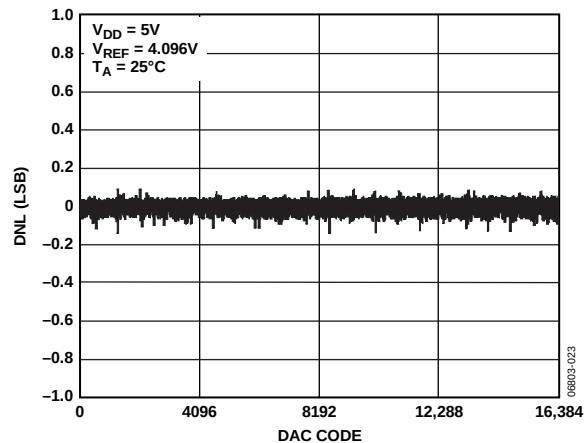
Figure 12. AD5044 DNL
