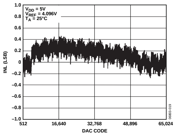
Figure 8. AD5064/AD5064-1 INL
