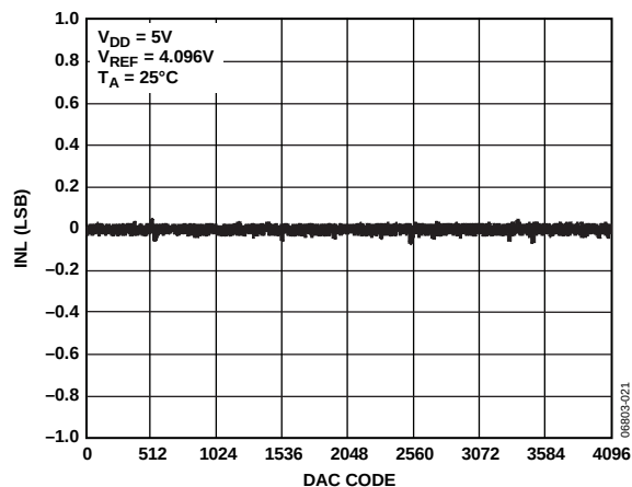
Figure 10. AD5024 INL
