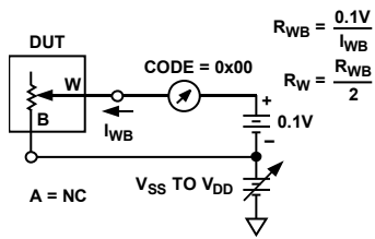
Figure 41. Wiper Resistance
