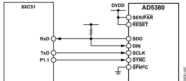
Figure 37. AD5380-to-8051 Interface
