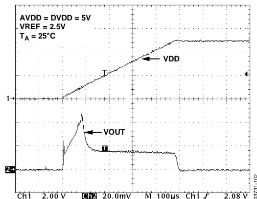
Figure 18. AD5380 Power-Up Transient
