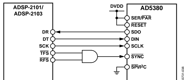
Figure 38. AD5380-to-ADSP-2101/ADSP-2103 Interface
