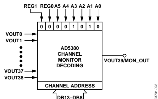
Figure 28. Channel Monitor Decoding
