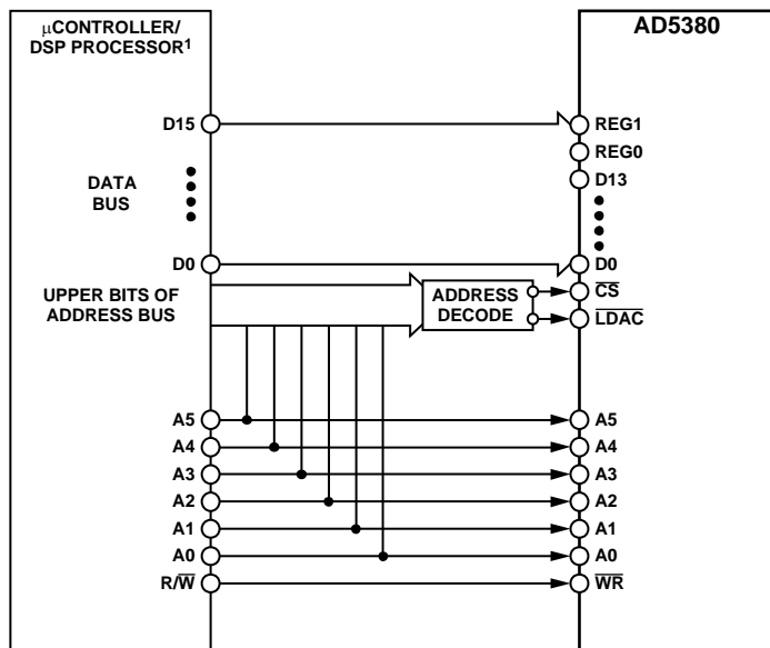
Figure 34. AD5380-to-MC68HC11 Interface
