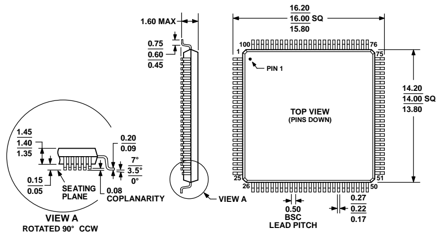
Figure 46. 100-Lead Low Profile Quad Flat Package [LQFP] (ST-100-1) Dimensions shown in millimeters
