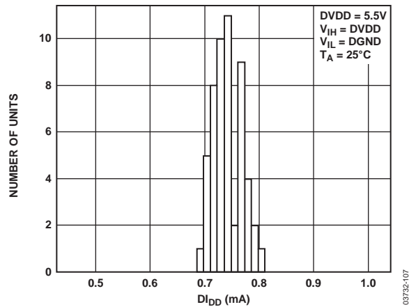
Figure 16. DI_{DD} Histogram
