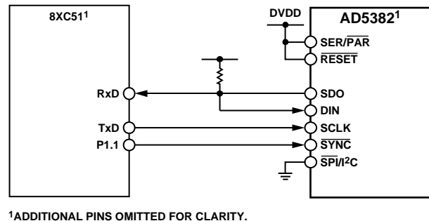
Figure 36. AD5382-to-8051 Interface
