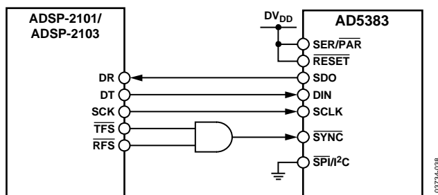
Figure 38. AD5383-to-ADSP-2101/ADSP-2103 Interface
