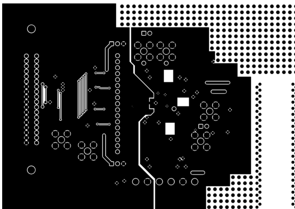
Figure 44. Solder-Side Artwork
