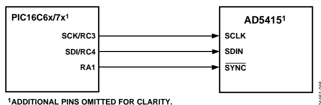
Figure 49. PIC16C6x/7x-to-AD5415 Interface
