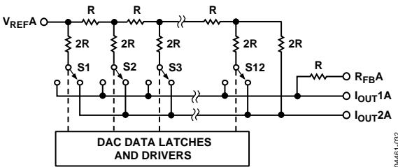
Figure 33. Simplified Ladder
