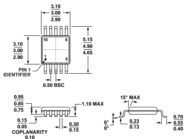
Figure 46. 10-Lead Mini Small Outline Package [MSOP] (RM-10) Dimensions shown in millimeters
