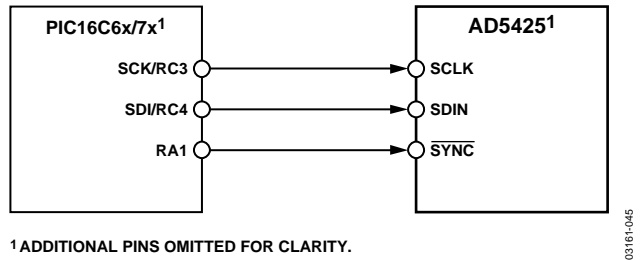
Figure 45. PIC16C6x/7x-to-AD5425 Interface
