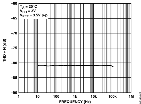
Figure 22. THD and Noise vs. Frequency
