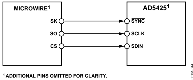
Figure 44. MICROWIRE-to-AD5425 Interface
