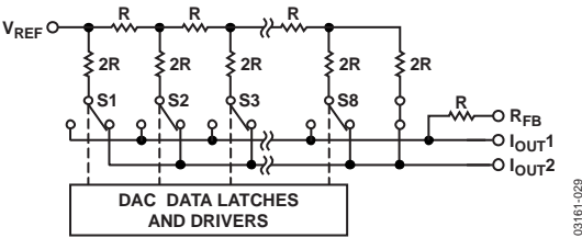
Figure 29. Simplified Ladder
