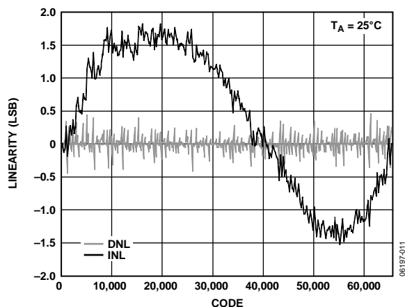
Figure 11. Force Current Linearity vs. Code, All Ranges, 1 LSB = 0.0015% FSR (20 V FSR)
