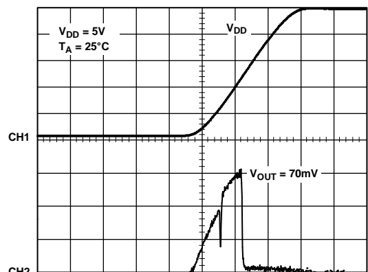
Figure 17. Power-On Reset to 0V
