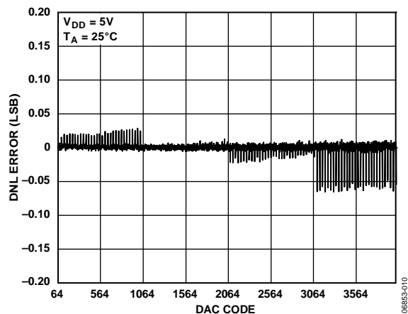
Figure 11. Typical AD5621 DNL
