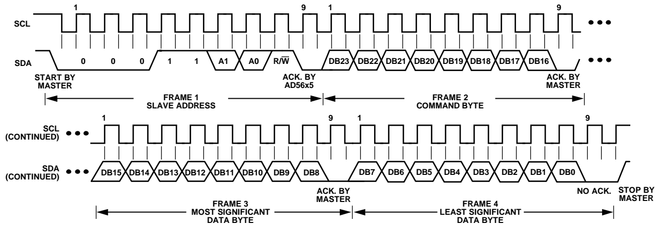
Figure 60. I²C Read Operation (10-Lead and 12-Ball Packages)
