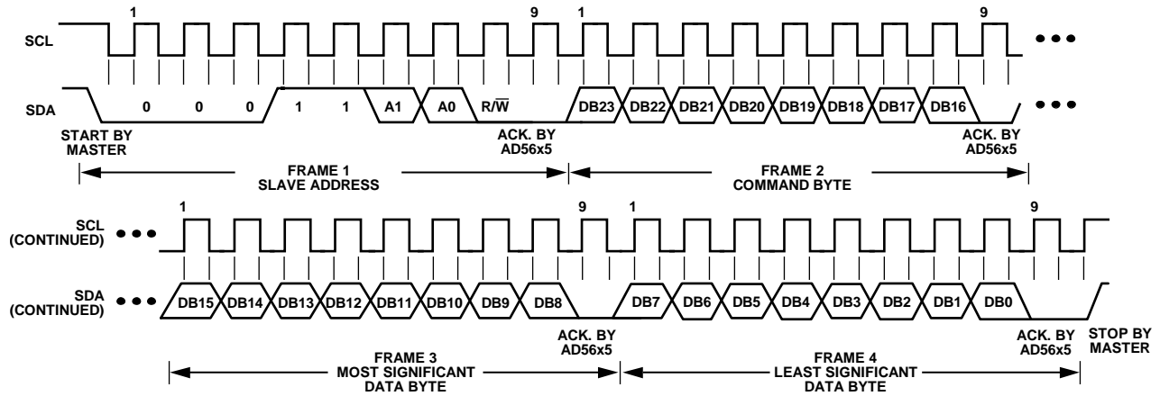
Figure 58. I²C Write Operation (10-Lead and 12-Ball Packages)
