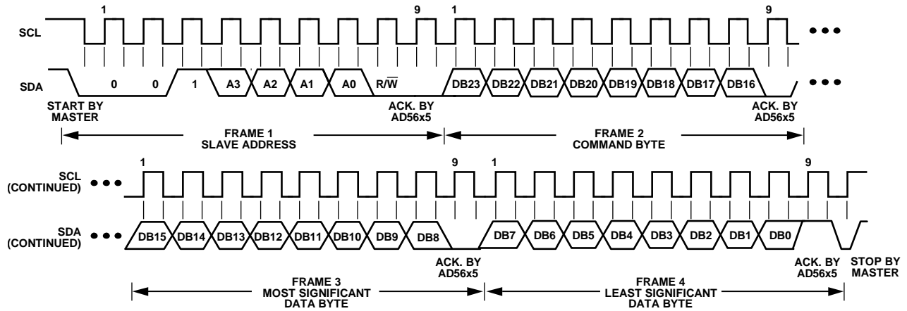
Figure 59. I²C Write Operation (14-Lead Package)
