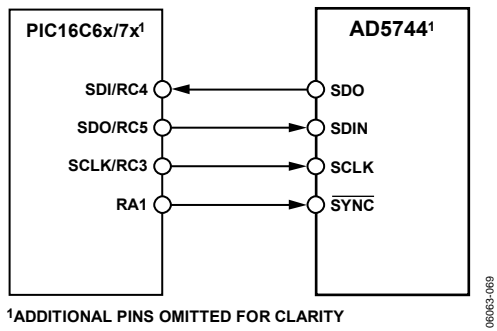
Figure 41. AD5744 to PIC16C6x/7x Interface
