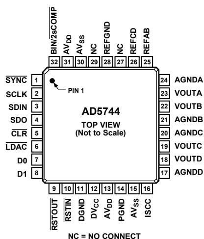
Figure 6. Pin Configuration
