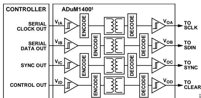
Figure 58. Isolated Interface
