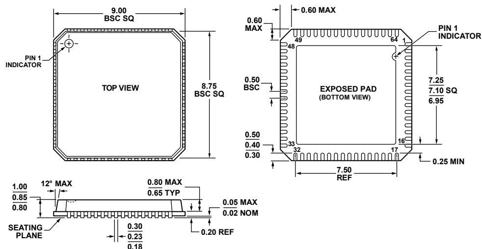
Figure 101. 64-Lead Lead Frame Chip Scale Package [LFCSP_VQ]
