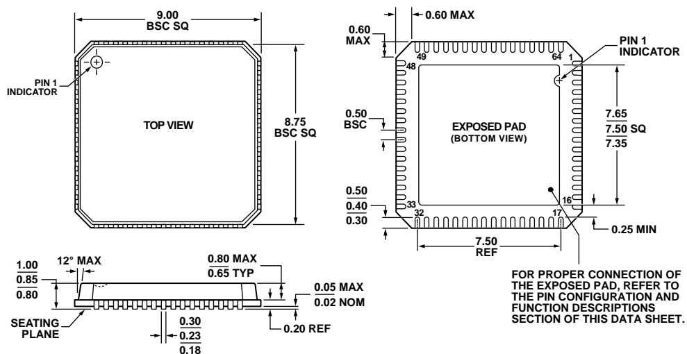
Figure 104. 64-Lead Lead Frame Chip Scale Package [LFCSP_VQ]
