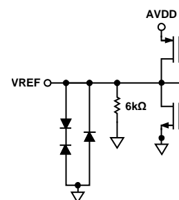
Figure 18. Equivalent VREF Circuit
