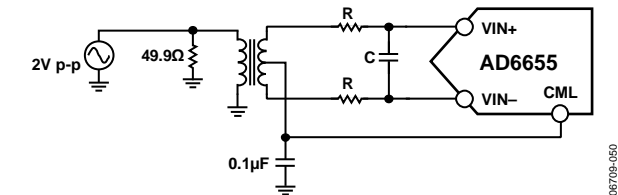
Figure 48. Differential Transformer-Coupled Configuration
