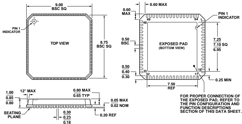
Figure 103. 64-Lead Lead Frame Chip Scale Package [LFCSP_VQ]
