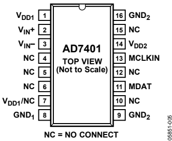
Figure 5. Pin Configuration
