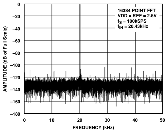
Figure 12. FFT Plot
