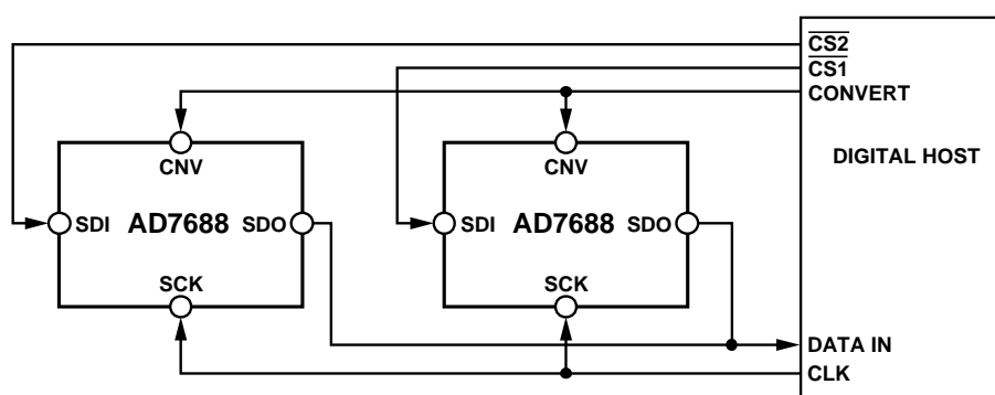
Figure 38. \overline{\text{CS}} Mode 4-Wire, No BUSY Indicator Connection Diagram
