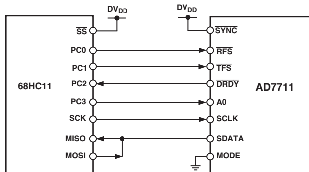
Figure 18. AD7711 to 68HC11 Interface
