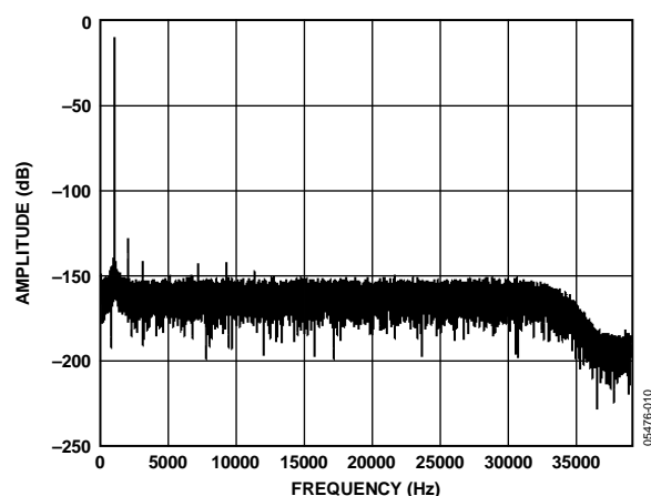
Figure 10. Low Power FFT, 1 kHz, -0.6 dB Input Tone, 256× Decimation
