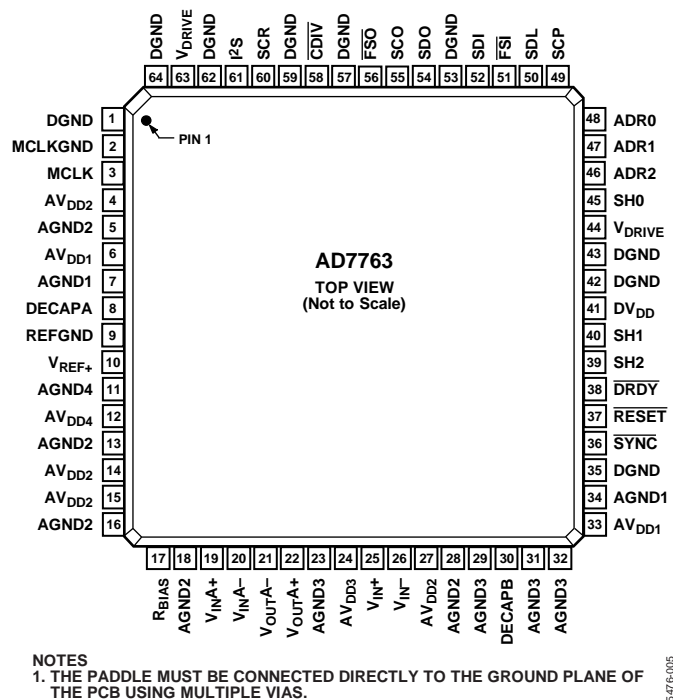
Figure 5. Pin Configuration
