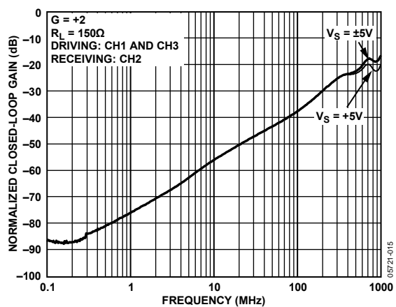
Figure 35. Worst-Case Crosstalk
