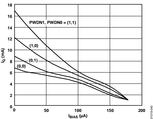
Figure 38. I_Q vs. I_{BIAS} Current; V_S = \pm 6V
