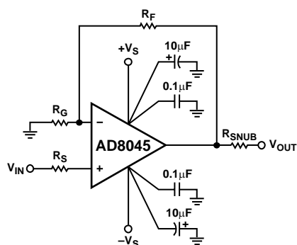
Figure 61. Noninverting Configuration
