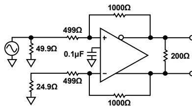
Figure 57. Basic Test Circuit, G = +2
