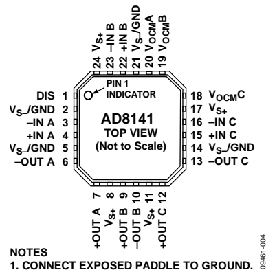
Figure 4. AD8141 Pin Configuration
