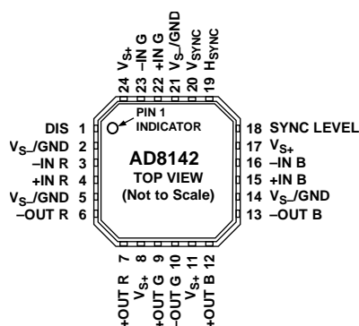
Figure 5. AD8142 Pin Configuration
