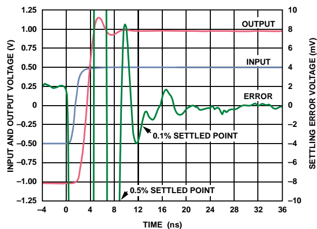
Figure 25. Differential Settling Time
