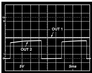
Figure 49. OUT1 Shorted to Ground, Square Wave Is OUT2, R_F = 1\text{ k}\Omega , R_G = 222\text{ }\Omega
