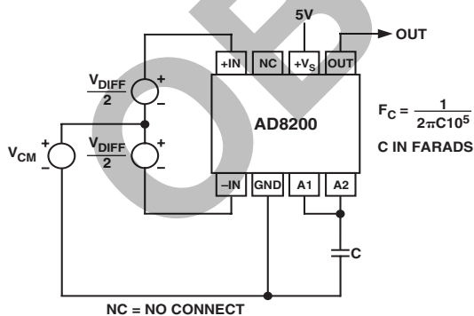
Figure 8. A Single-Pole, Low-Pass Filter Using the Internal 100\text{ k}\Omega Resistor
