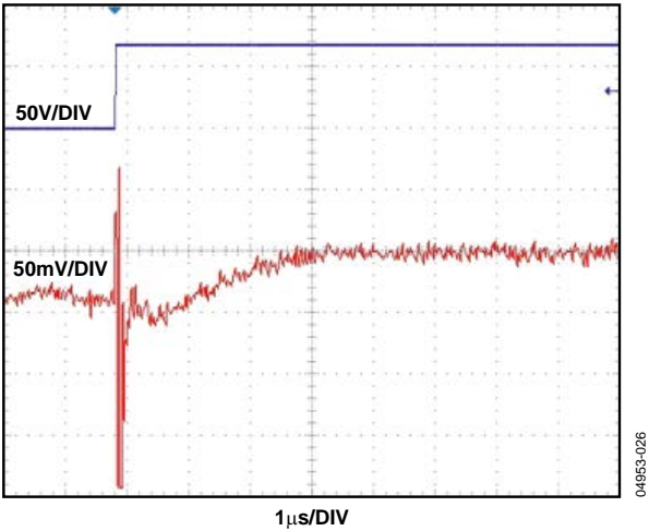
Figure 12. Common-Mode Response
