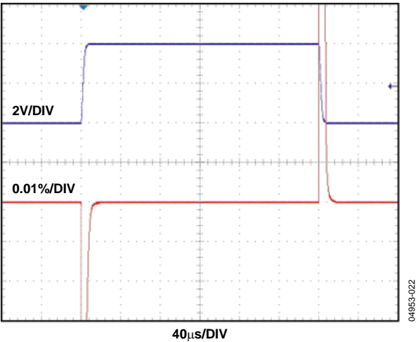
Figure 11. Settling Time
