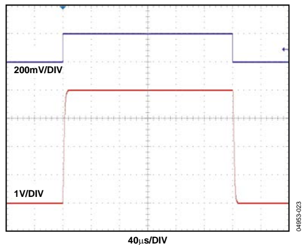
Figure 8. Rise/Fall Time
