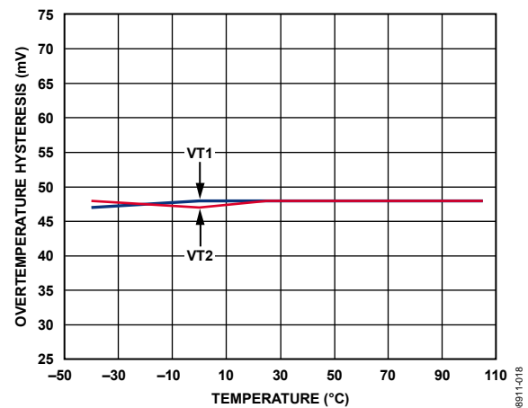
Figure 20. Overtemperature Hysteresis vs. Temperature
