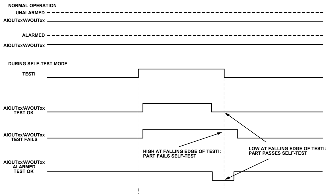
Figure 51. Timing Diagram for Alarms at AIOUxx and AVOUTxx
