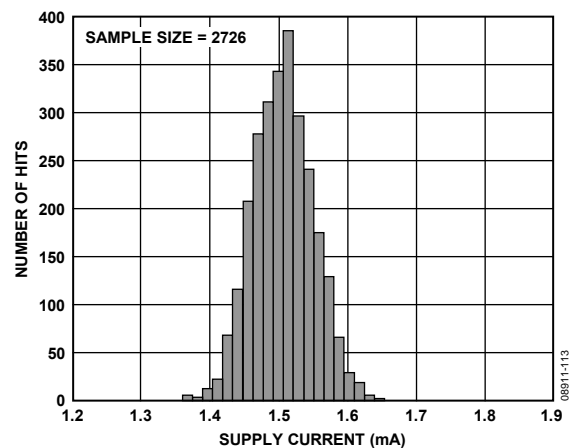
Figure 13. Supply Current
