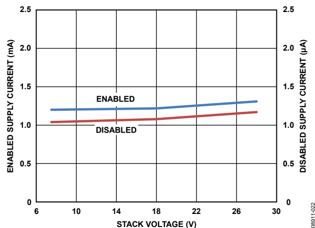
Figure 24. Supply Current vs. Stack Voltage (VIN6 – VIN0)
