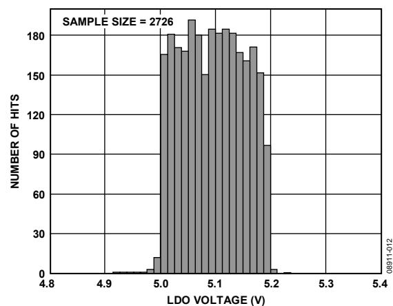
Figure 12. LDO Voltage
