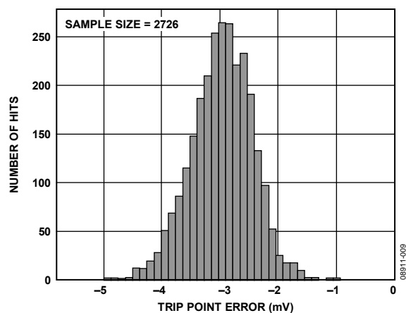
Figure 9. Overtemperature Trip Point Error
