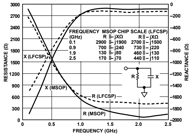
Figure 11. Input Impedance
