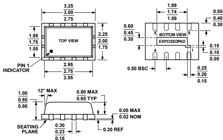
Figure 47. 8-Lead Lead Frame Chip Scale Package [LFCSP_VD] 2 mm x 3 mm Body, Very Thin, Dual Lead (CP-8-1)
