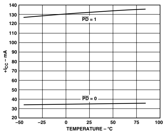
TPC 12. Supply Current vs. Temperature
