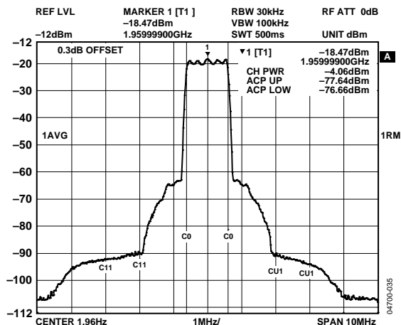
Figure 35. Output Spectrum, 1960 MHz, Single-Carrier CDMA2000 Test Model at -4 dBm, V_{\text{BBI}} = V_{\text{BBQ}} = 0.353 V, Adjacent Channel Power Measured at \pm 2.25 MHz Carrier Offset in 1 MHz BW Input Signal Filtered Using a Cavity Tuned Filter (Pass Band = 6.8 MHz)
