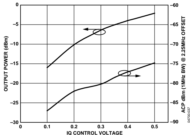
Figure 37. Output Power and ACP vs. I and Q Control Voltages, CDMA2000 Test Model, V_{\text{BBI}} = V_{\text{BBQ}} , ACP Measured at \pm 2.25 MHz Carrier Offset in 1 MHz BW
