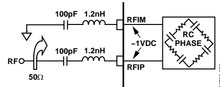
Figure 29. RF Input Interface to the AD8341 Showing Coupling Capacitors and Matching Inductors
