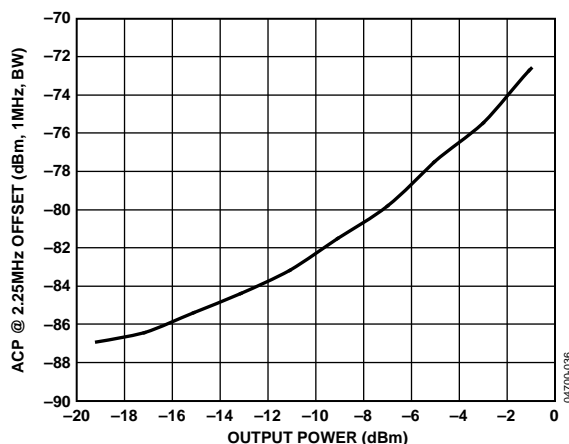
Figure 36. Adjacent Channel Power vs. Output Power, CDMA2000 Single Carrier @ 1960 MHz; ACP Measured at \pm 2.25 MHz Carrier Offset (1 MHz BW); V_{\text{BBI}} = V_{\text{BBQ}} = 0.353 V
