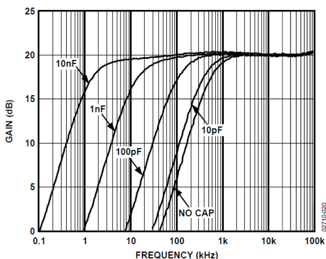
Figure 9. Gain vs. Frequency for Multiple Values of HPFL Capacitor at V_{GAIN} = 500mV .
