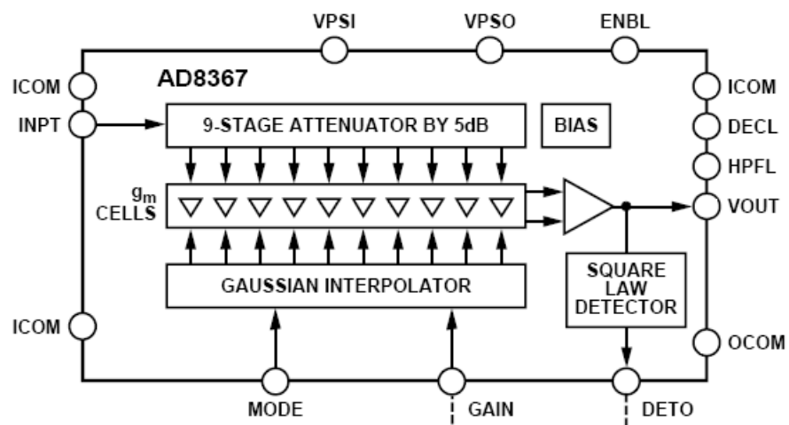
Figure 2 – Block Diagram.
