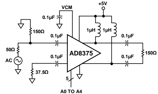
Figure 33. Single-Ended-to-Differential Conversion
