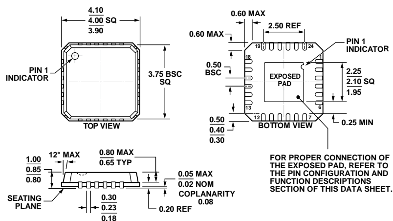
Figure 51. 24-Lead Lead Frame Chip Scale Package [LFCSP_VQ] 4 mm × 4 mm Body, Very Thin Quad (CP-24-1) Dimensions shown in millimeters
