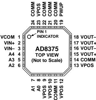
Figure 3. Pin Configuration
