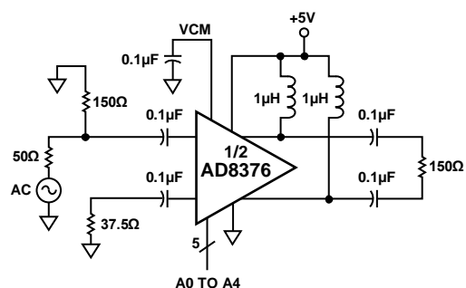
Figure 34. Single-Ended-to-Differential Conversion Featuring ½ of the AD8376
