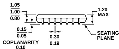
Figure 36. 14-Lead Thin Shrink Small Outline Package [TSSOP] (RU-14)
