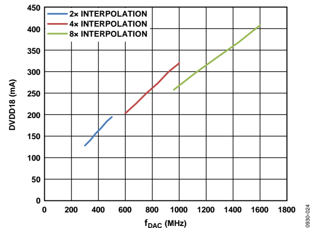
Figure 25. DVDD18 Current vs. f_{DAC} over Interpolation
