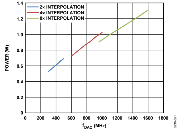
Figure 24. Total Power Consumption vs. f_{DAC} over Interpolation
