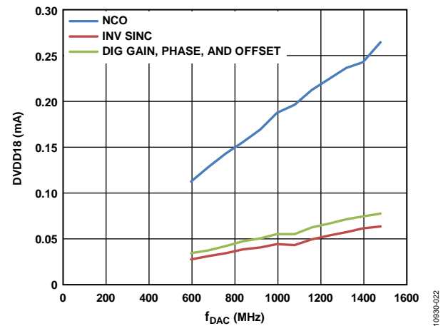
Figure 26. DVDD18 Current vs. f_{DAC} over Digital Functions
