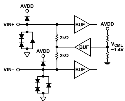
Figure 34. Analog Inputs ( V_{CM} \approx 1.4\text{ V} )
