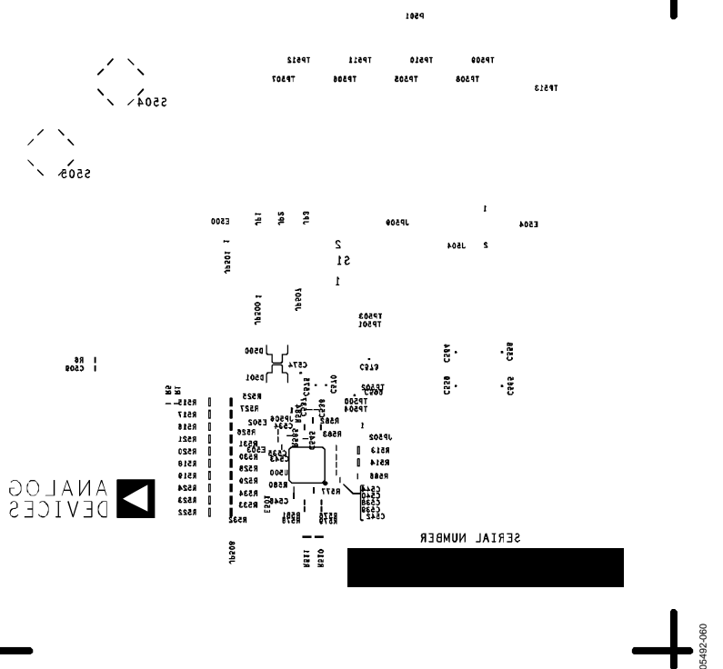
Figure 70. Evaluation Board Layout, Silkscreen Secondary Side (Mirrored Image)
