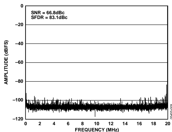
Figure 9. AD9237-40 20 MHz FFT
