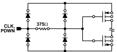
Figure 7. Equivalent CLK, PDWN Input Circuit
