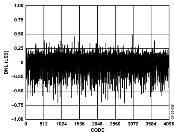
Figure 31. Typical DNL
