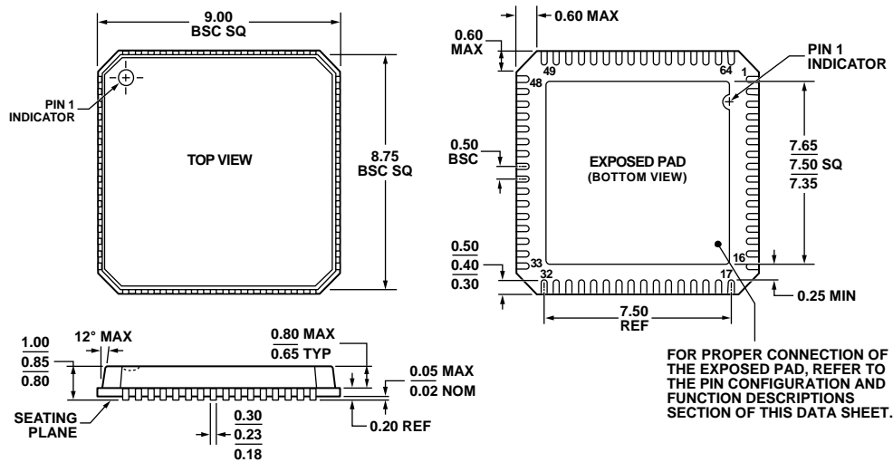
Figure 85. 64-Lead Lead Frame Chip Scale Package [LFCSP_VQ]
