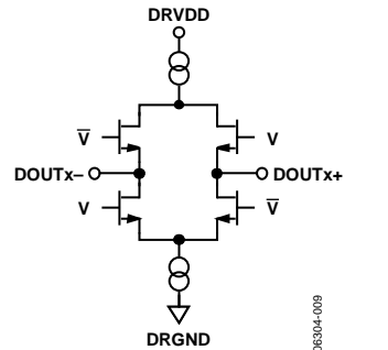
Figure 9. Equivalent Digital Output Circuit
