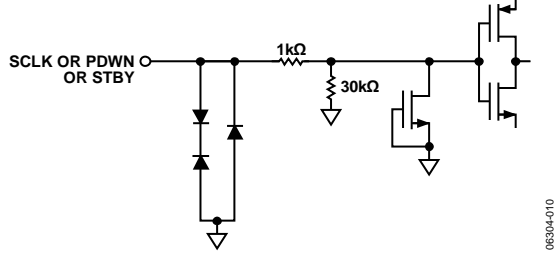
Figure 10. Equivalent SCLK Input Circuit
